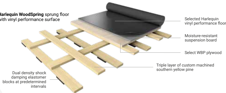
Harlequin WoodSpring sprung floor with solid hardwood or engineered board surface
